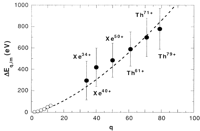
FIG. 3. Evaluated energy gains \Delta E_{q,im} due to image charge attraction for Xe^{q+} and Th^{q+} projectiles vs charge state q (full symbols). Comparison is made with data for Xe^{q+} ( q \leq 12 ) impact on Fe ([20], open symbols) as well as the prediction of the COB model (staircase approximation [27], dotted line).
