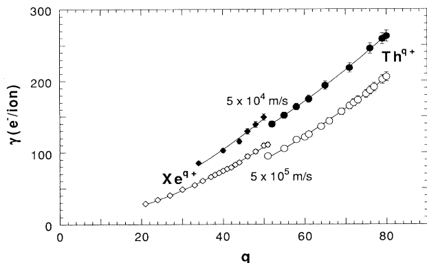
FIG. 1. Measured total electron yields vs charge state q for ^{136}\text{Xe}^{q+} ( 21 \leq q \leq 51 , diamonds) and ^{232}\text{Th}^{q+} ( 51 \leq q \leq 80 , circles) impact on a clean gold surface at 5 \times 10^4 m/s (filled symbols) and 5 \times 10^5 m/s (open symbols) impact velocity, respectively.
