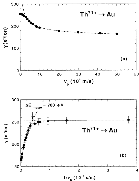
FIG. 2. (a) Measured total electron yield \gamma vs nominal (cf. text) projectile velocity v_p for impact of ^{232}\text{Th}^{71+} on clean polycrystalline gold. (b) Same as (a) but plotted vs the inverse nominal projectile velocity, in order to quantify the image charge effect (cf. text). Dashed curve gives electron yields extrapolated according to Eq. (2).
