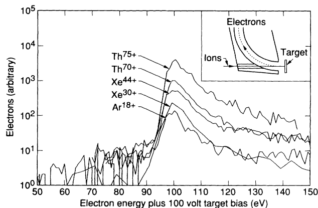
FIG. 1. Electron emission spectra following \text{Ar}^{18+} , \text{Xe}^{30+} , \text{Xe}^{44+} , \text{Th}^{70+} , and \text{Th}^{75+} impact at normal incidence on Au. Inset: Target-area geometry. The ions approach from the left to the target on the right; the electrons move to the left and up to the detector (not shown).
